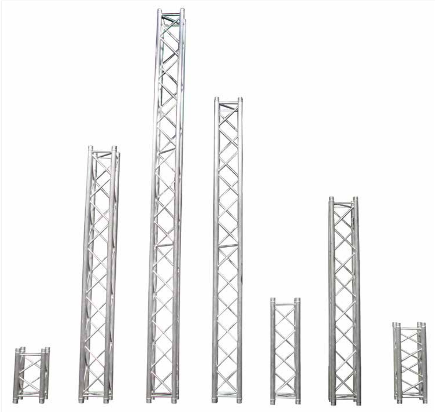
Prolyte H30V 0.5m, 0.75m, 1.0m, 2.0m, 2.5m, 3.0m, 4.0m 1000587.00, 1001010.00, 1000588.00, 1000589.00, 1000590.00, 1000591.00, 1003321.00
