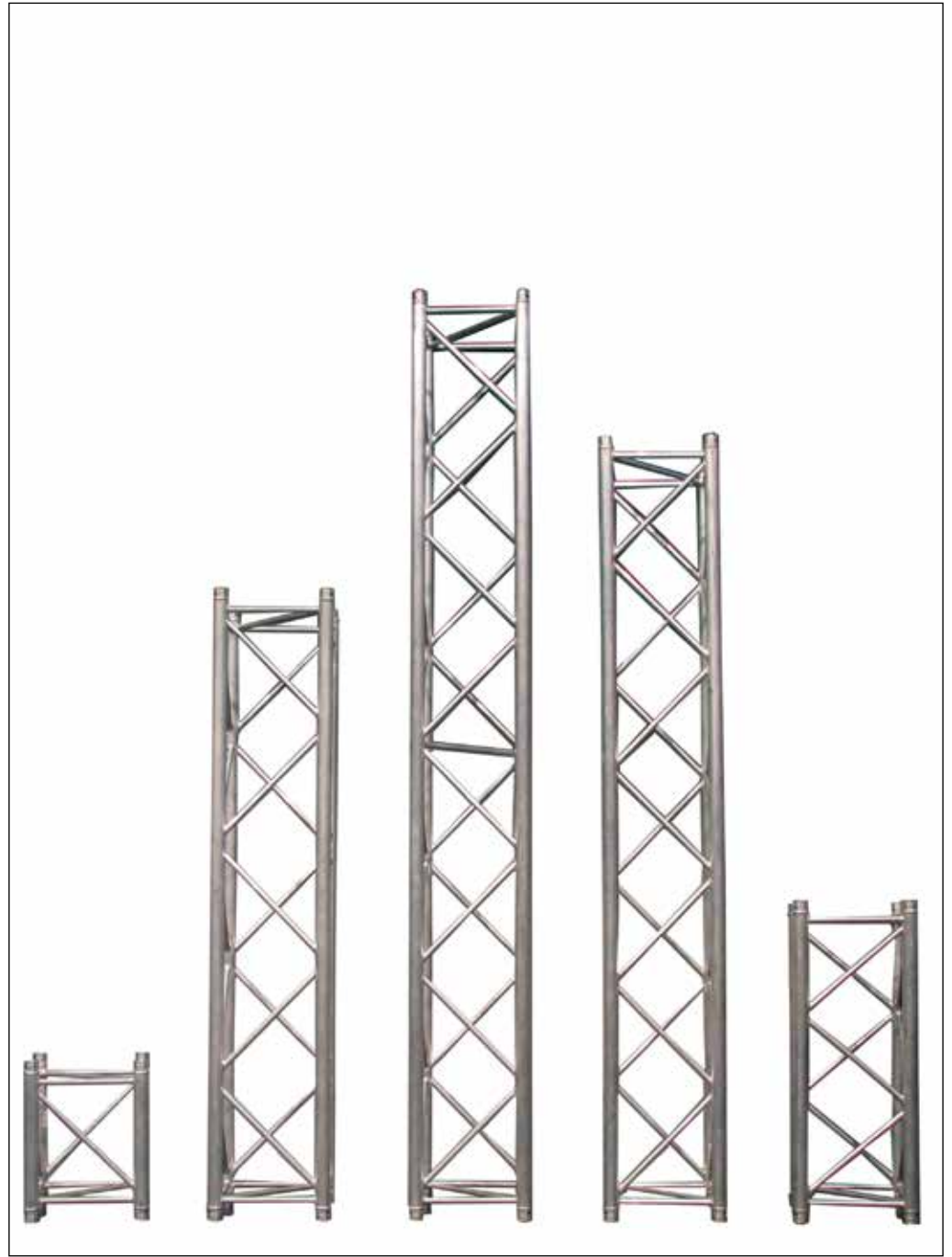
Prolyte H40V 0.5m, 1.0m, 2.0m, 2.5m, 3.0m 1001007.00, 1000585.00, 1001008.00, 1000586.00, 1001009.00
